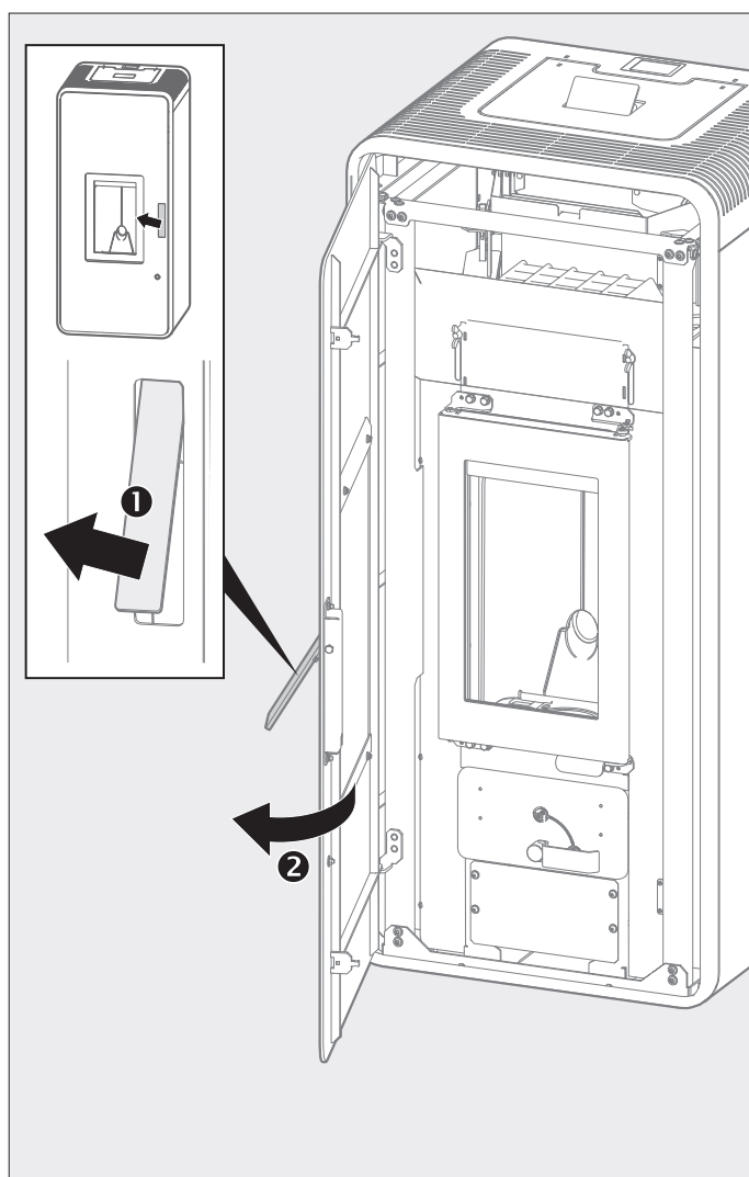
Fig. 3.10 Opening and closing the door
