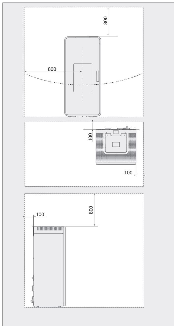
Fig. 2.5 Distances minimales
