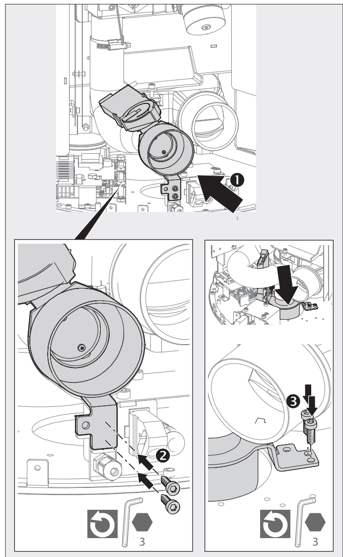
Fig. 2.16 Install the lower back wall and panel supplied
