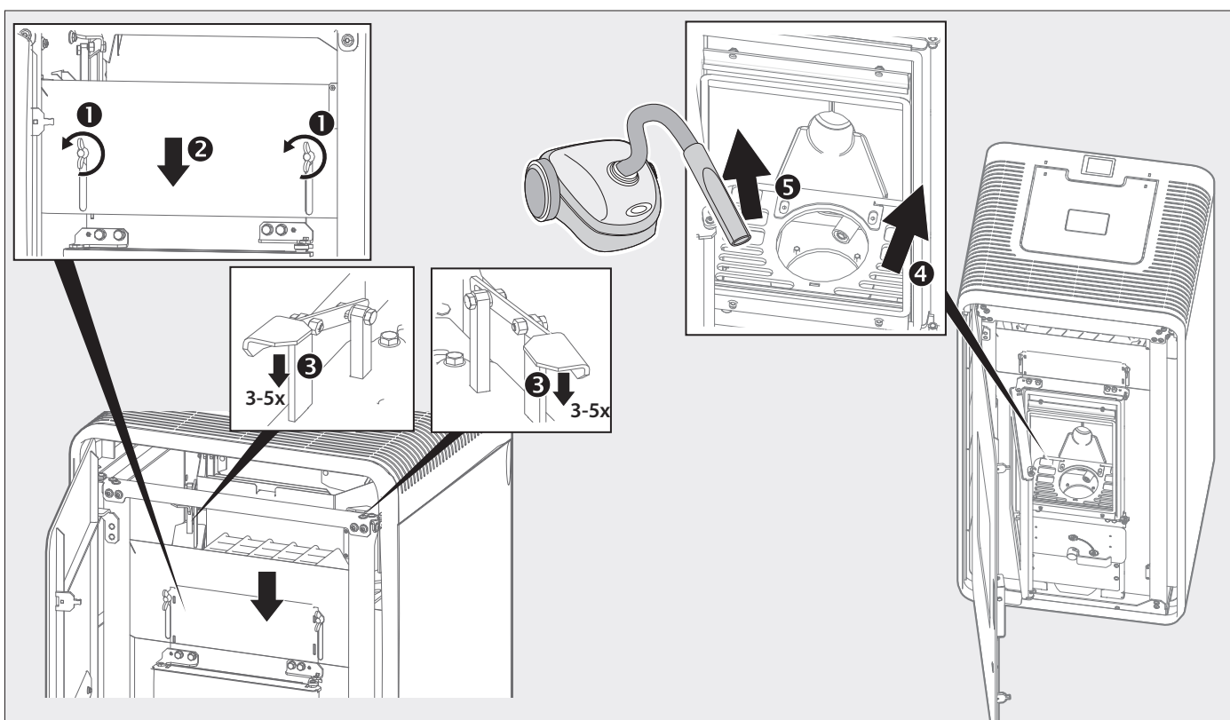
Abb. 4.2 Cleaning the combustion chamber – operating the cleaning slides
