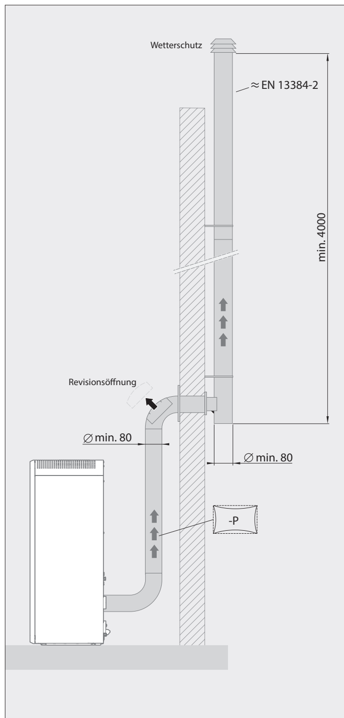
Fig. 2.6 Exhaust gas connection
