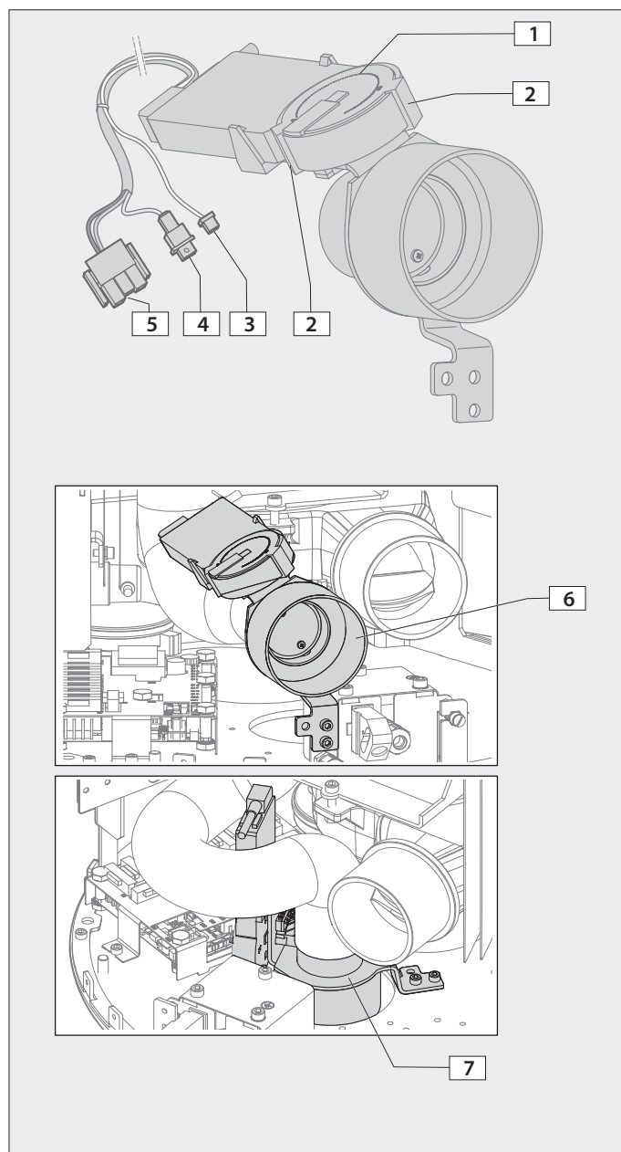
Fig. 2.13 Connection of a motor-driven combustion air damper
