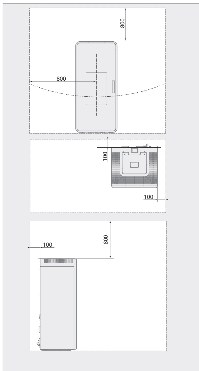
Abb. 2.5 Minimum distances
