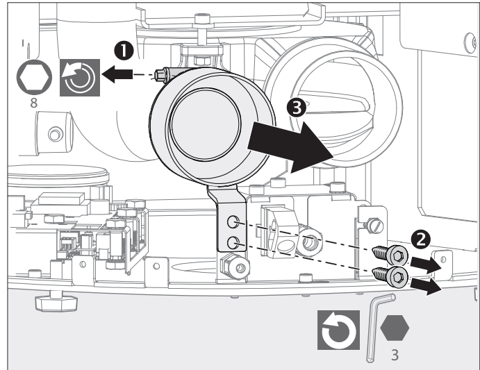
Fig. 2.15 Unscrew the combustion air nozzles
