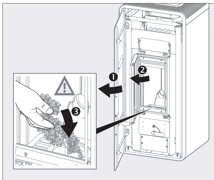
Fig. 2.23 Pour pellets in manually if the pellet duct is empty
