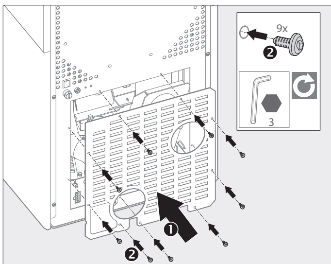
Fig. 2.17 Install the lower back wall
