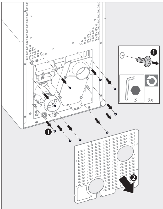
Fig. 2.9 Remove the lower back wall and panel
