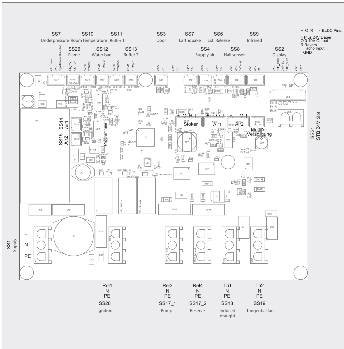
Fig. 2.22 Electrical connection diagram
