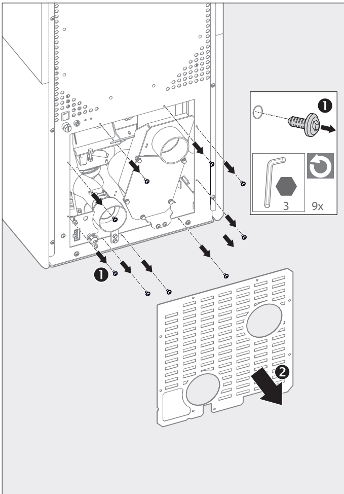
Fig. 2.14 Remove the lower back wall
