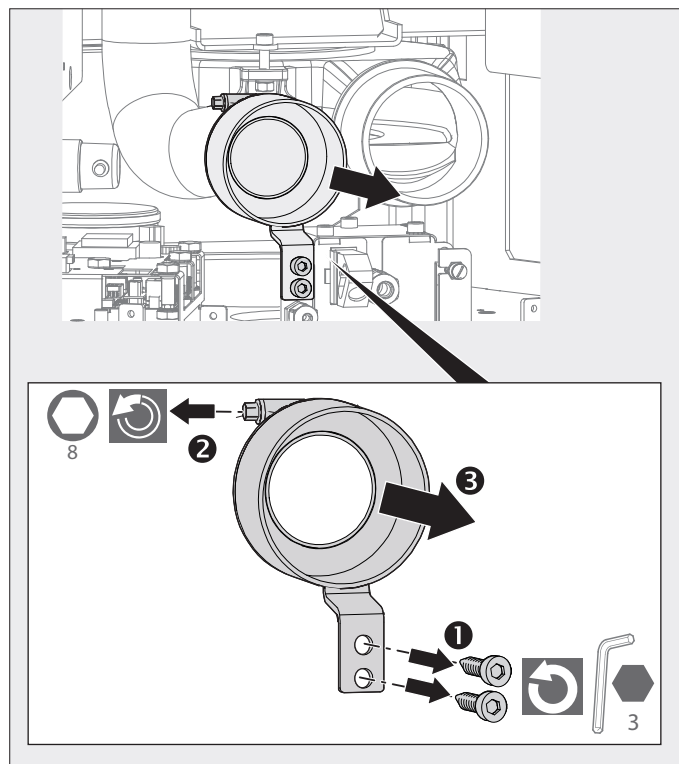
Fig. 2.10 Unscrew the combustion air nozzles
