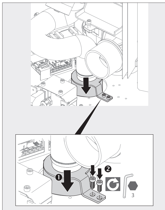
Fig. 2.11 Screw the combustion air nozzles onto the base plate
