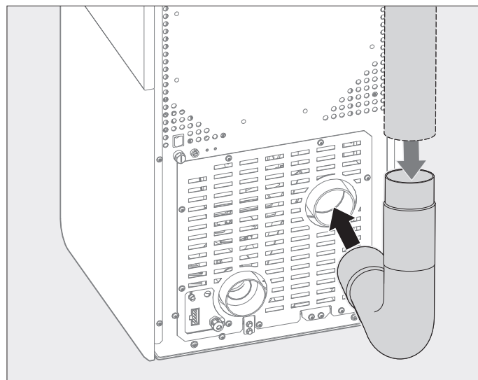
Fig. 2.7 Plug the exhaust pipe (on site) into the connection
