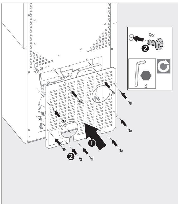
Fig. 2.12 Install the lower back wall
