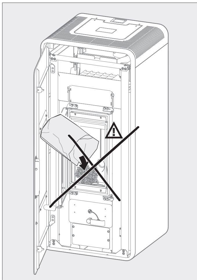
Fig. 3.7 Do not manually pour pellets into the burner trough except if the reservoir has run empty
