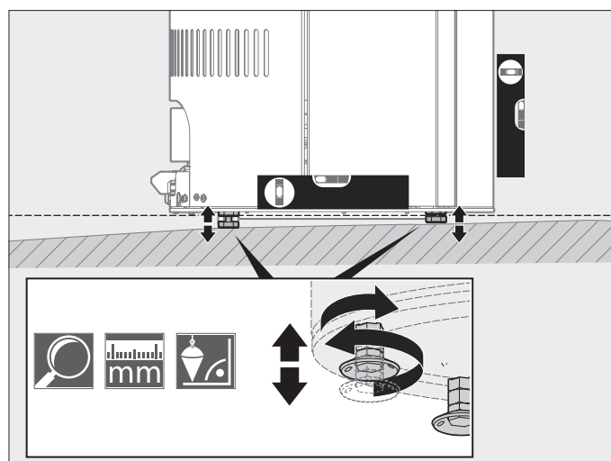
Fig. 2.21 Adjust the pellet fireplace with the adjusting feet
