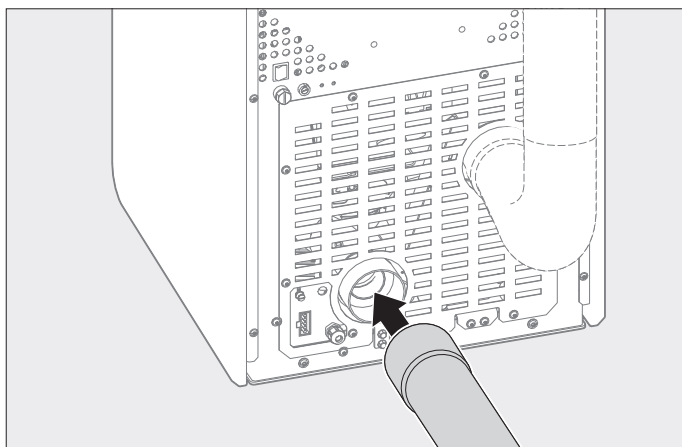
Fig. 2.8 Plug the Ø 80 mm combustion air line into the rear
