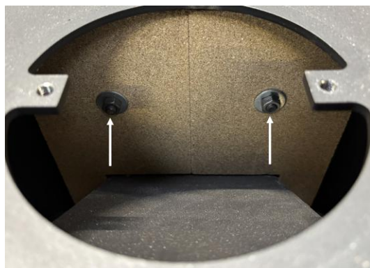
3) Remove the two nuts inside the burning chamber.
